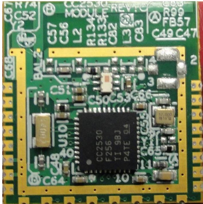
EUT with Shield Opened
