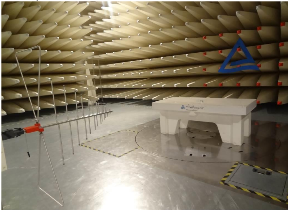
Test setup
