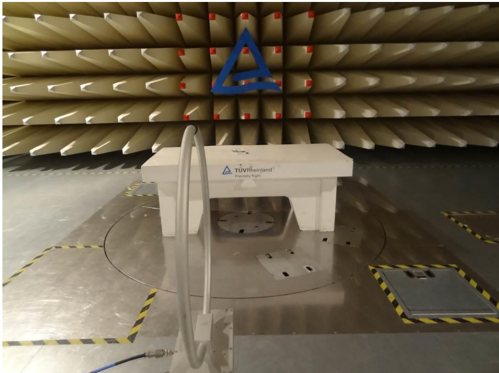
Test setup
