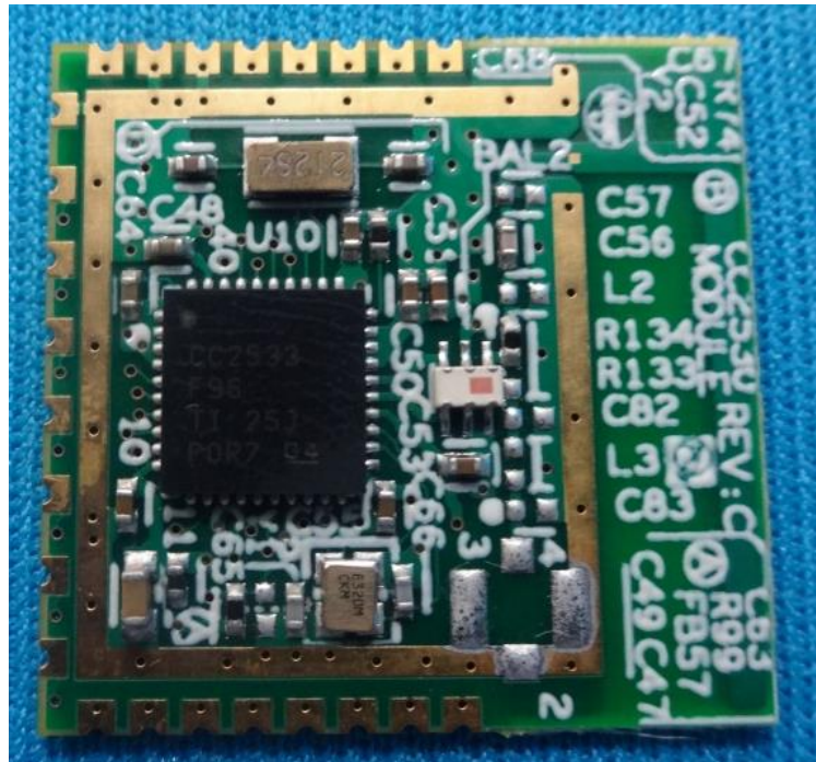
EUT with Shield Opened
