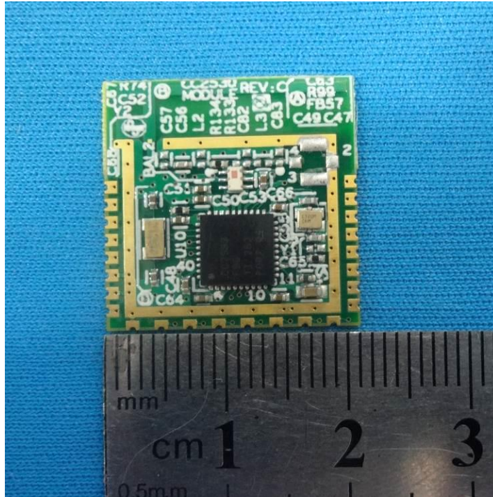
EUT Dimensional View
