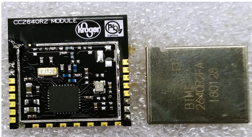
Photo 2: RF Module with shielding removed
