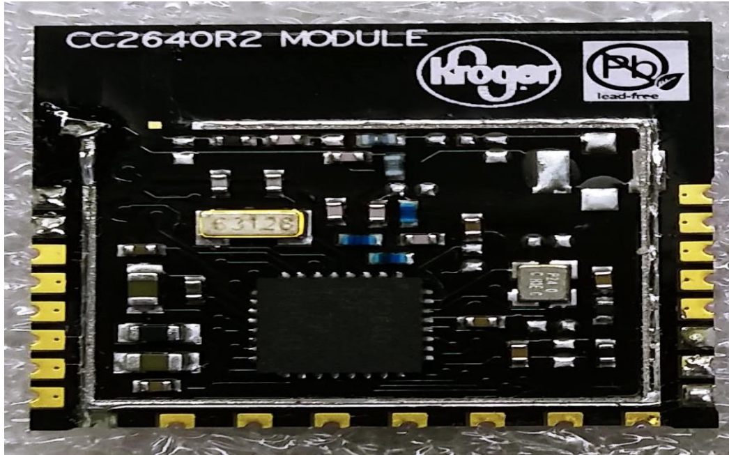
Photo 1: RF Module Front view
