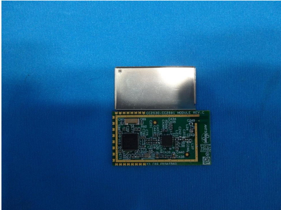
Module With Shielding Removed
