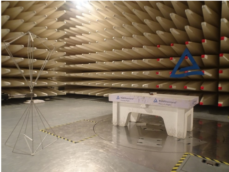
Vertical Polarization
