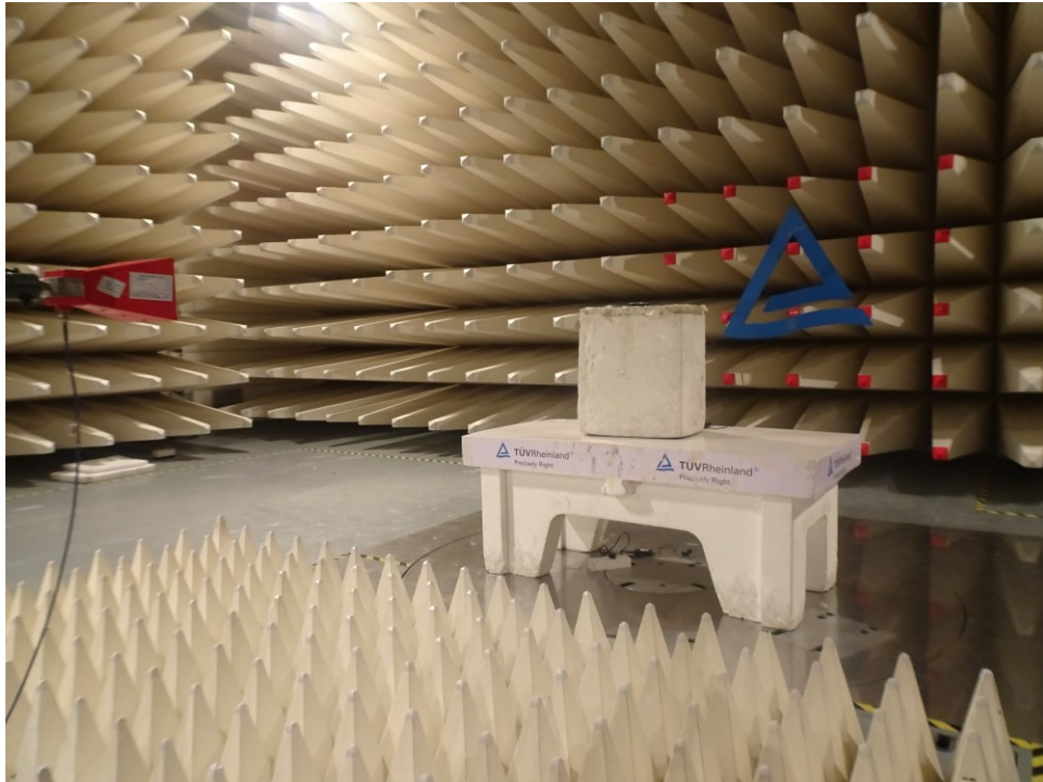
Vertical Polarization
