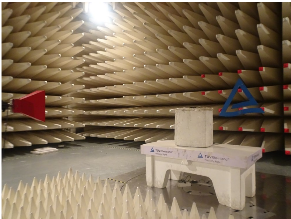
Horizontal Polarization
