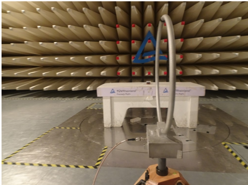
Perpendicular Polarization
