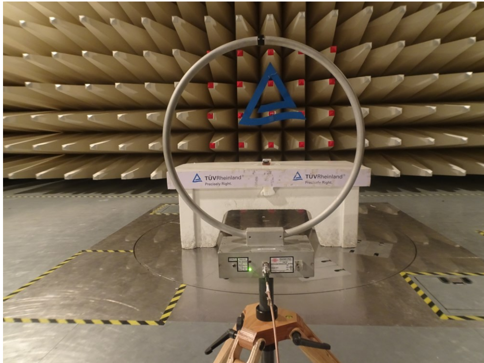
Parallel Polarization
