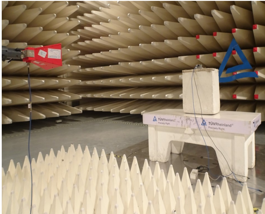
Vertical Polarization
