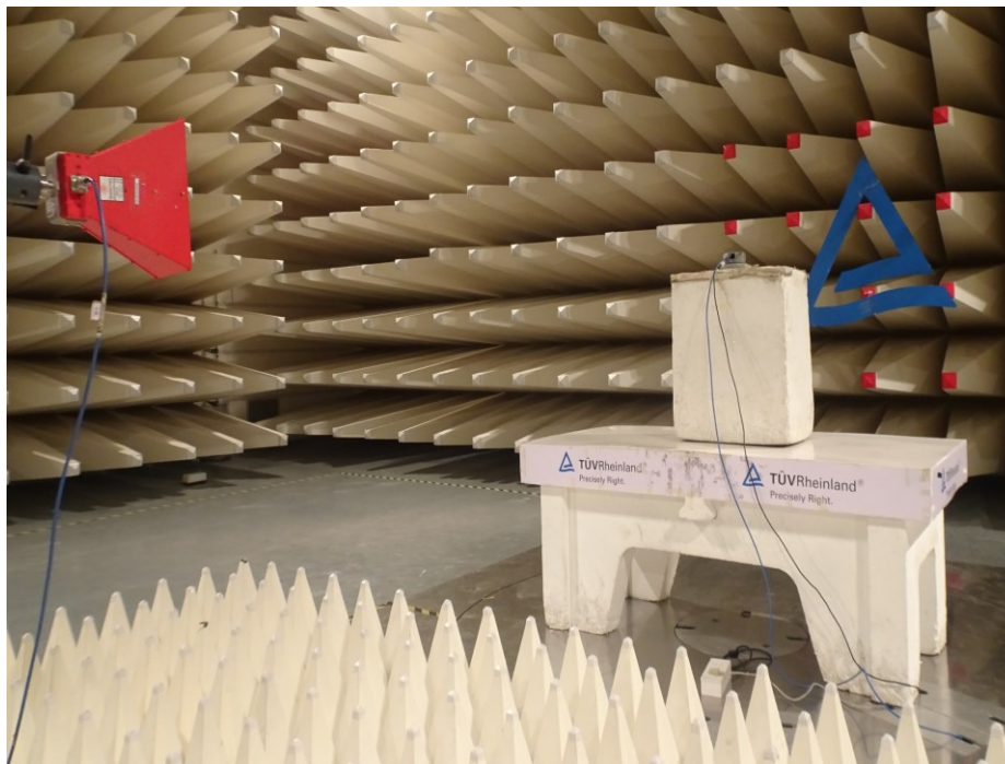
Horizontal Polarization
