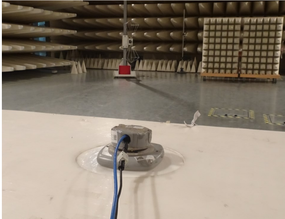
Vertical Polarization
