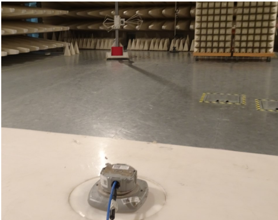
Horizontal Polarization
