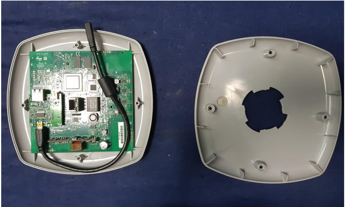
EUT Panel Removed
