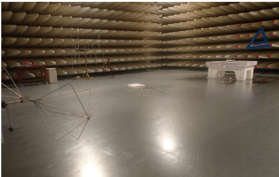
Photo 4: Biconical antenna Horizontal polarization
