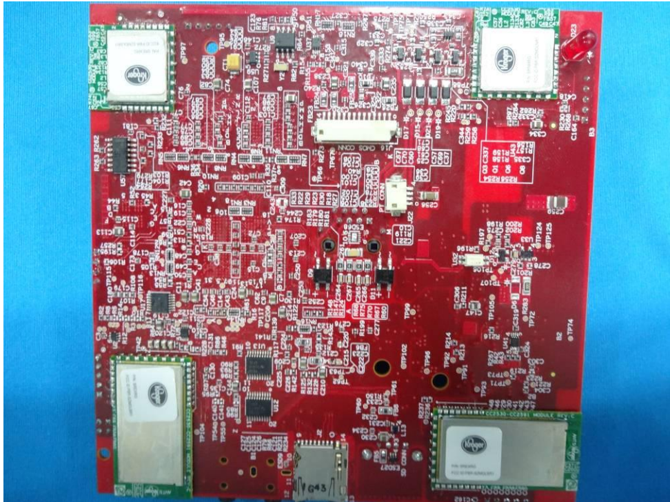
Bottom View Of Internal PCB
