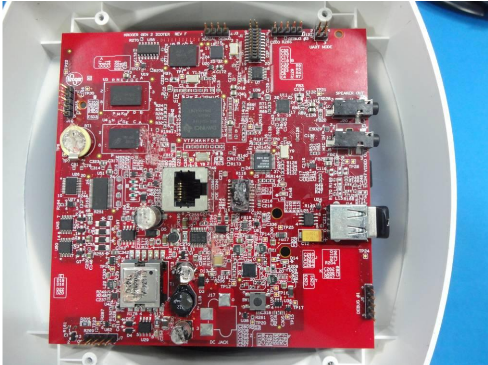
EUT With Bottom Enclosure Removed
