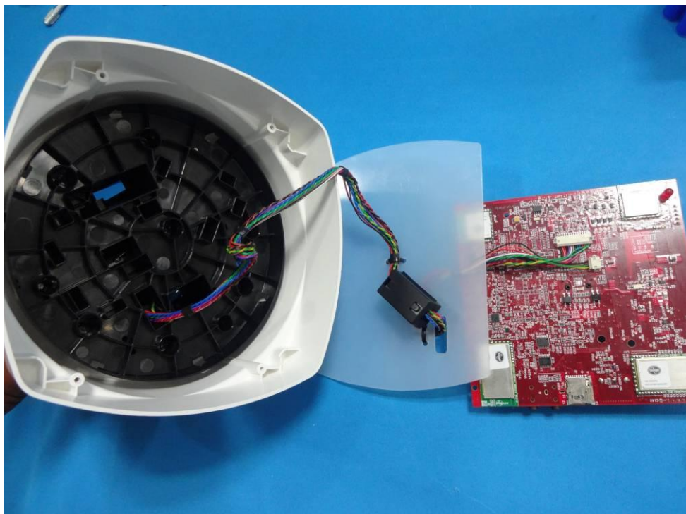
EUT With Bottom PCB Removed
