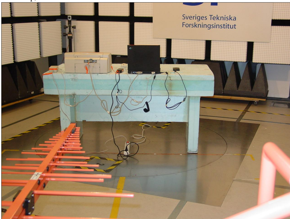
Test set-up, Radiated emission
