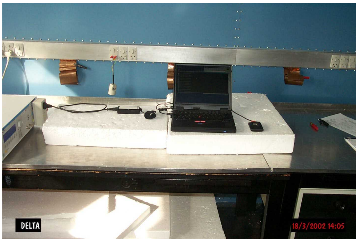
Photo A2.5 Burst transient test
