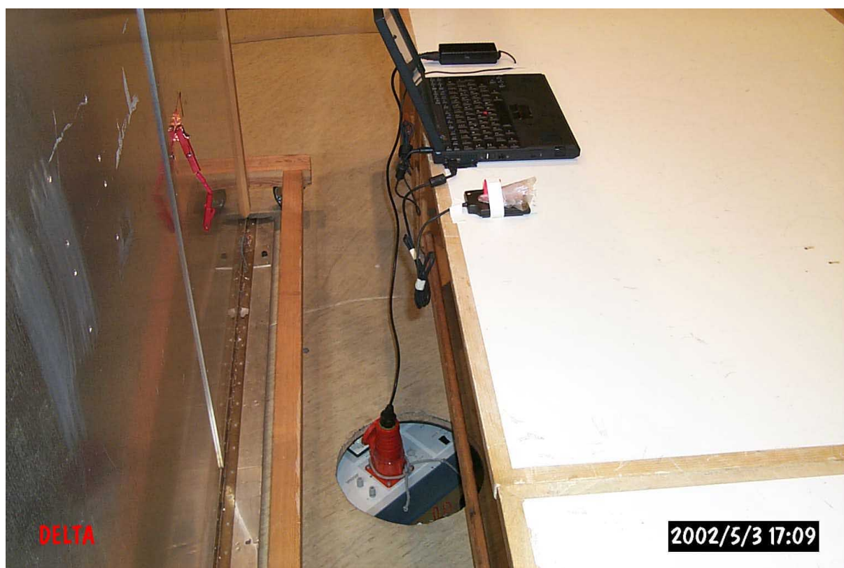
Photo A6.4 AC mains conducted emission. Test object in fingerprint scanning mode
