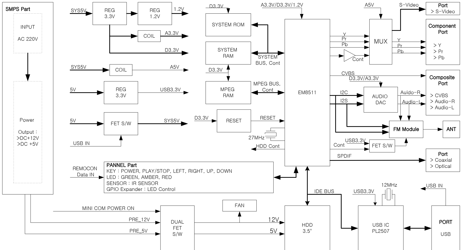
DVP-370 BLOCK DIAGRAM
