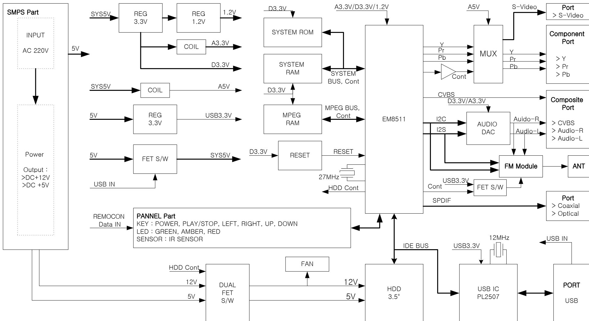
DVP-355 BLOCK DIAGRAM
