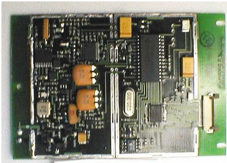
RF Module Shield Removed
