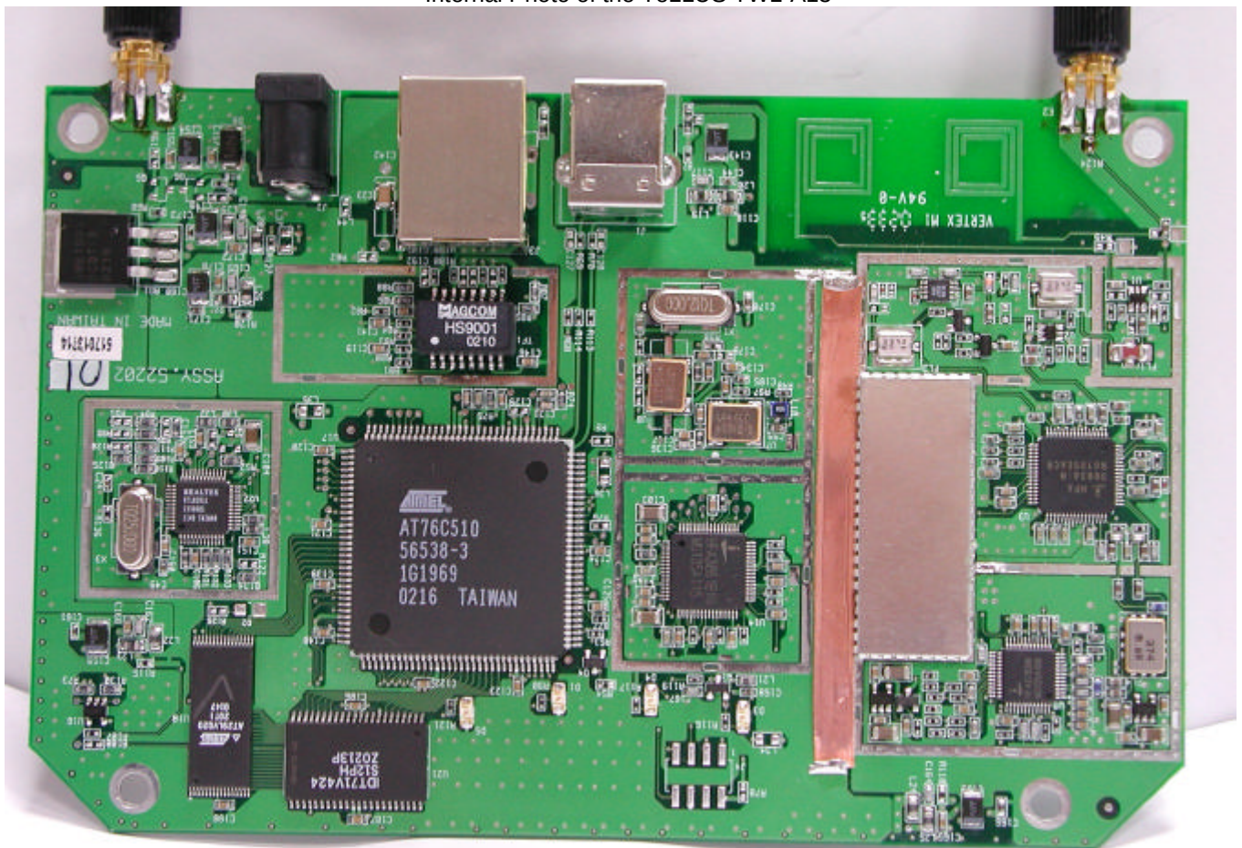
Internal Photo of the TeLLUS TWL-A13
