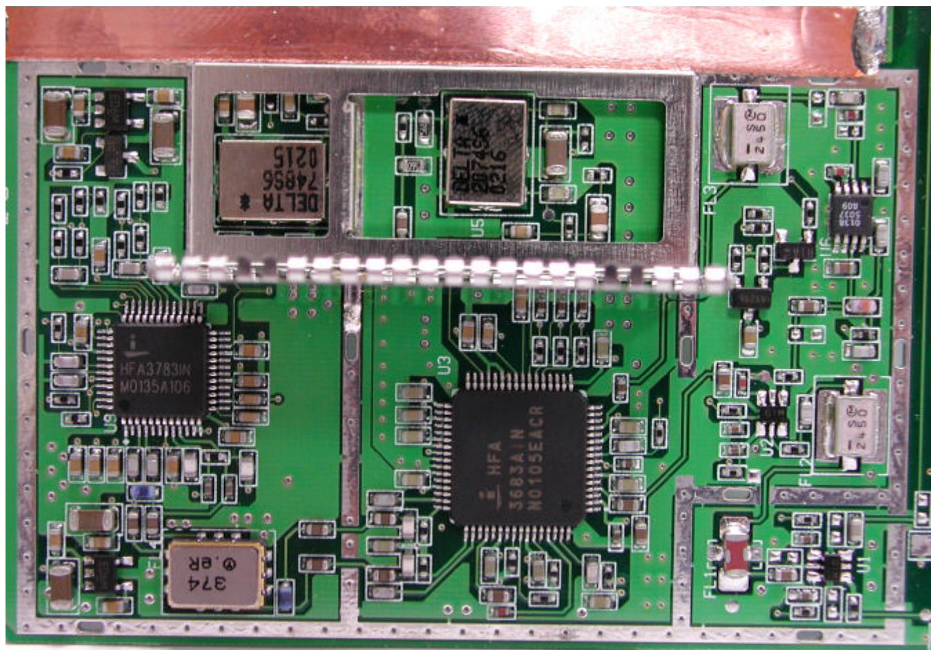
Internal Photo of the TeLLUS TWL-A13
