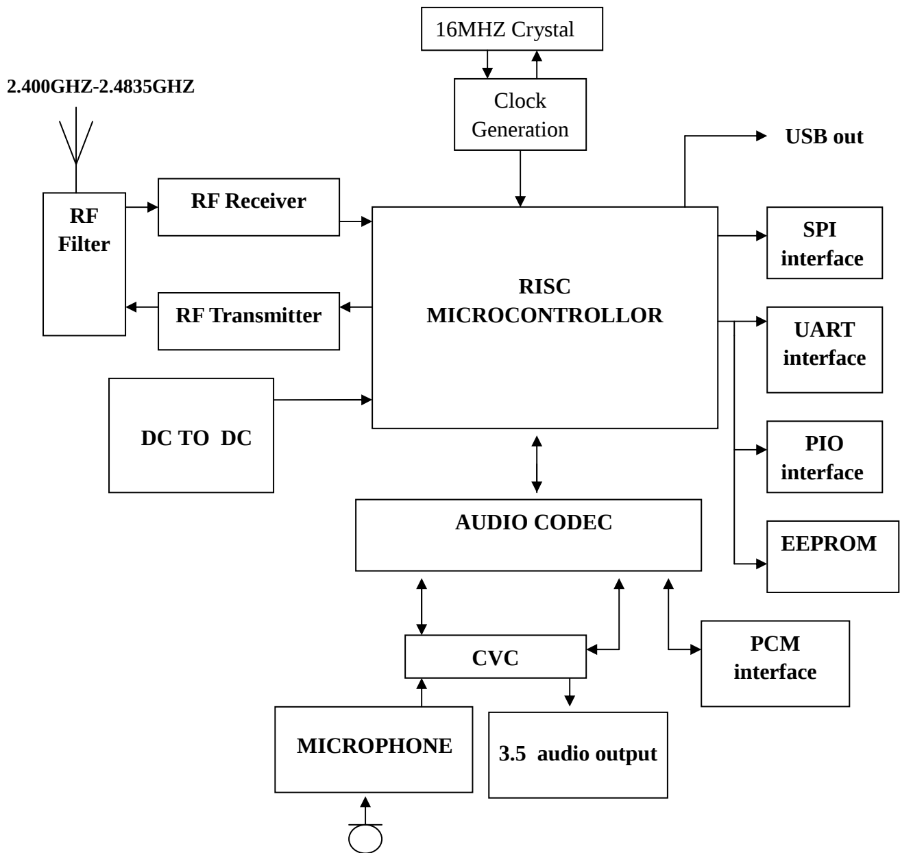
PI-1101BH Block Diagram
