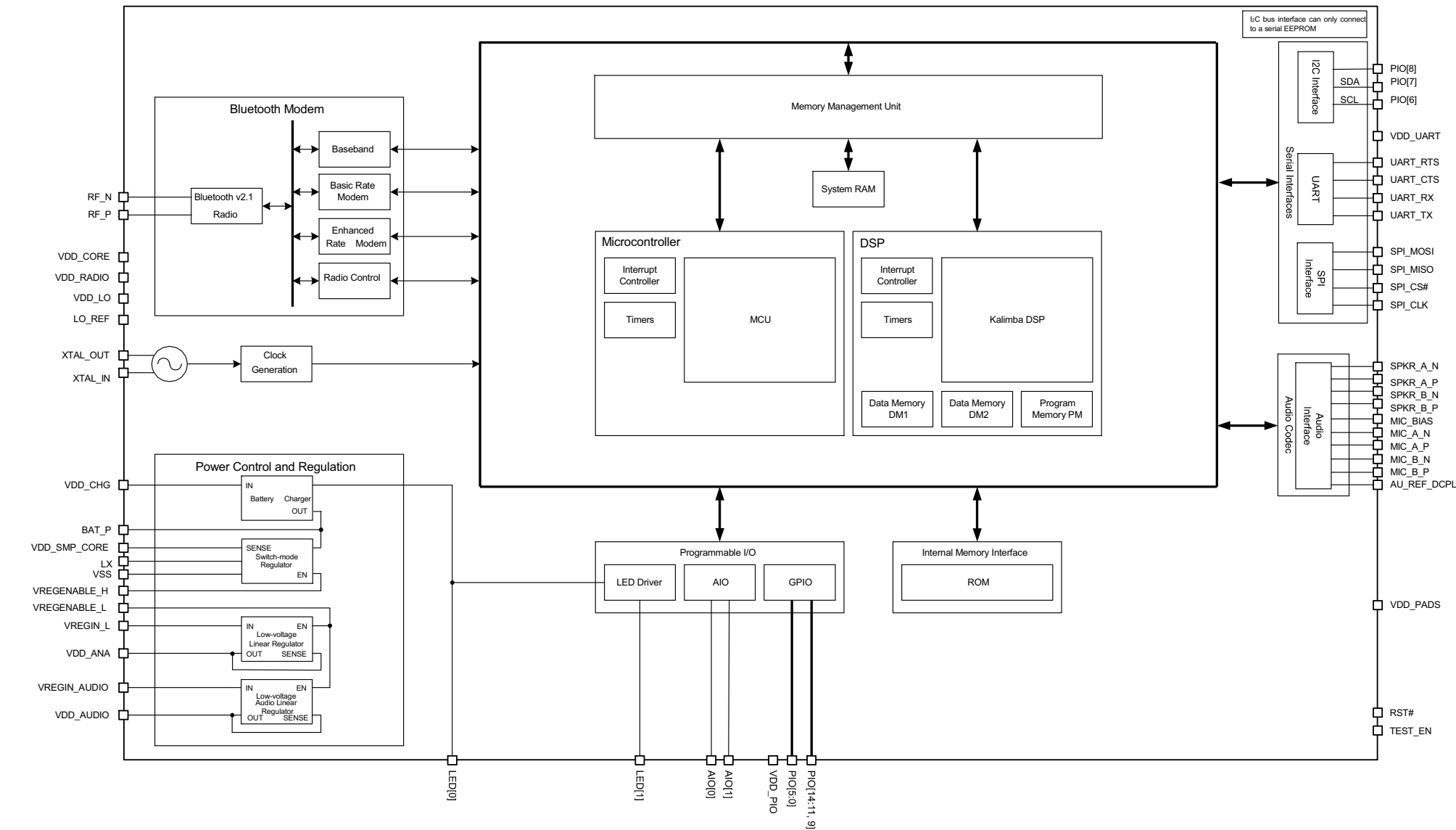
BC57F687A05 Block Diagram
