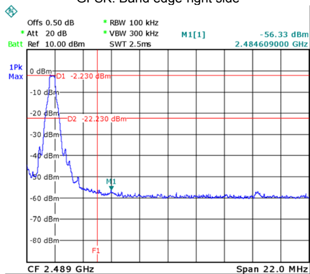
GFSK: Band edge-right side
