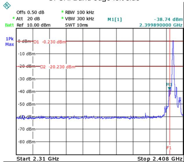
GFSK: Band edge-left side
