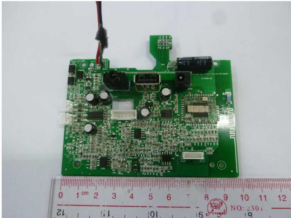
PCB1 View
