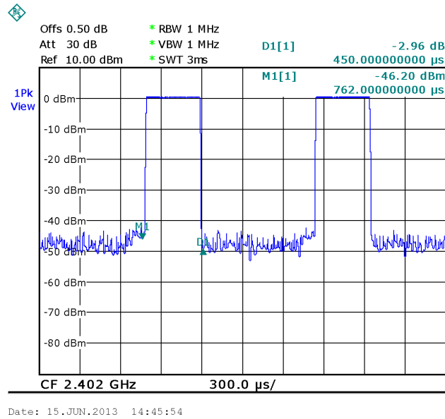
(b) Single pulse time is 0.45ms
