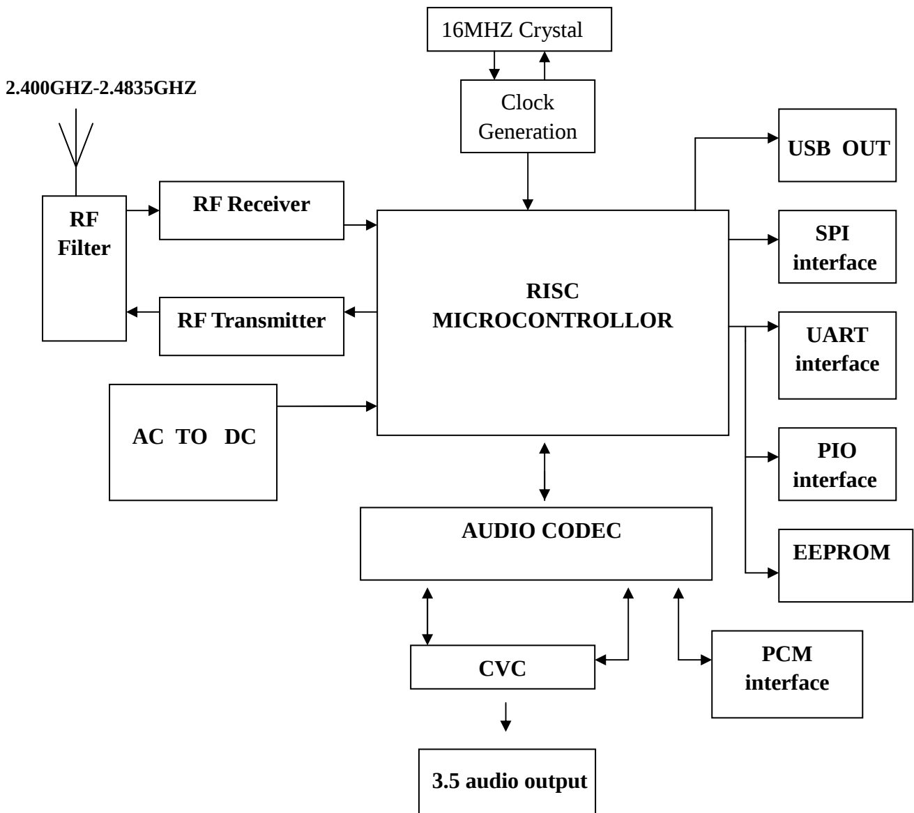
TC-1072BT Block Diagram
