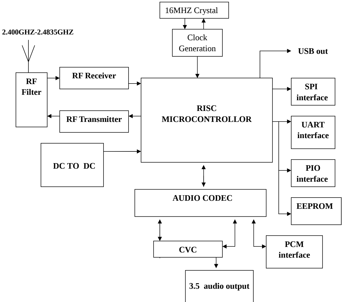
PI-1101BH Block Diagram
