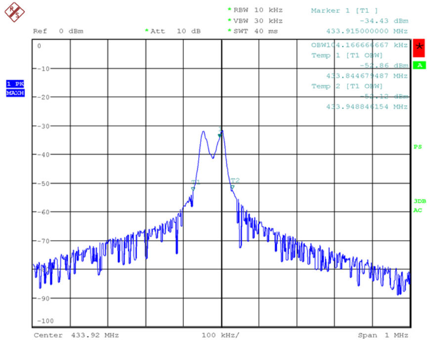
Plot 1: 99% Occupied bandwidth
