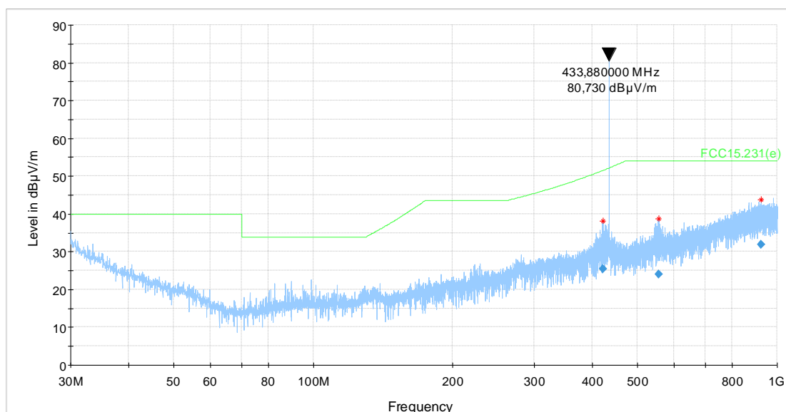
Plot 1: 30 MHz to 1000 MHz, vertical & horizontal polarisation
