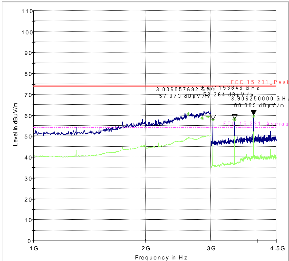
FCC 15.231 1-4.5GHz_TX
