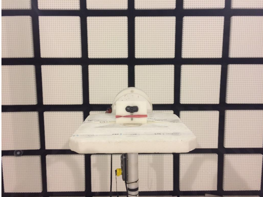
Photo 5: RSE set-up 1 GHz to 6 GHz
