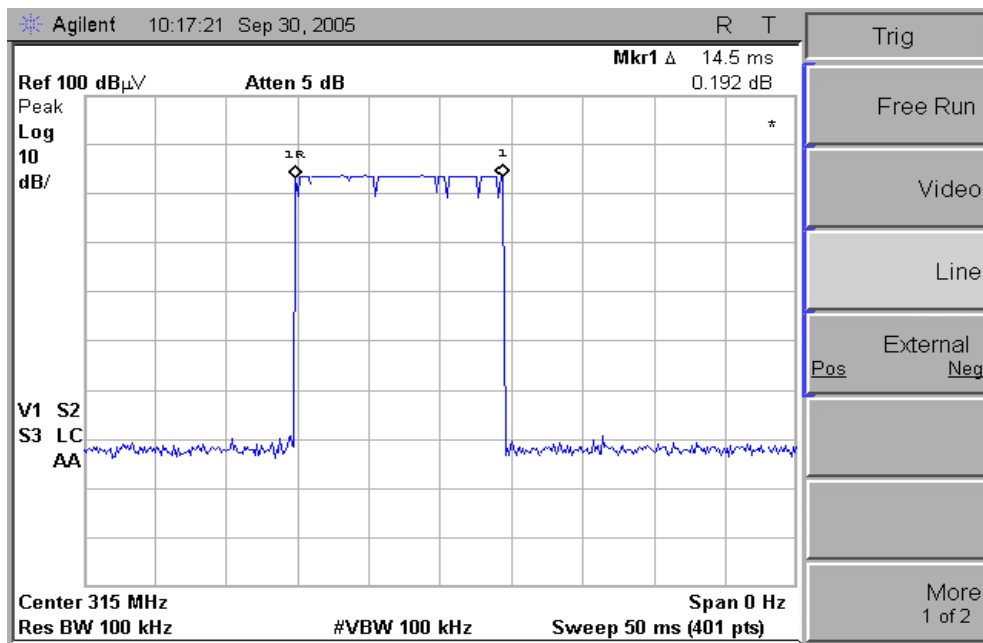
Figure 1. normal transmission
