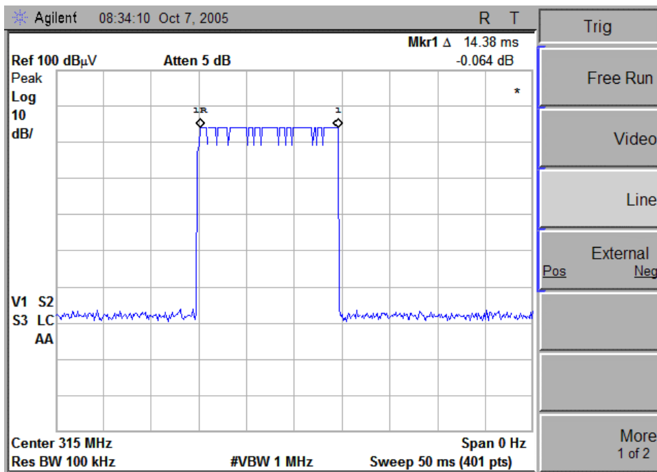
Figure 1. normal transmission
