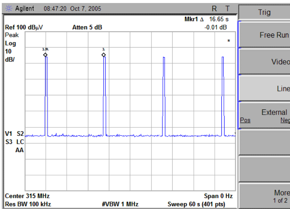
Figure 4. Transmission interval
