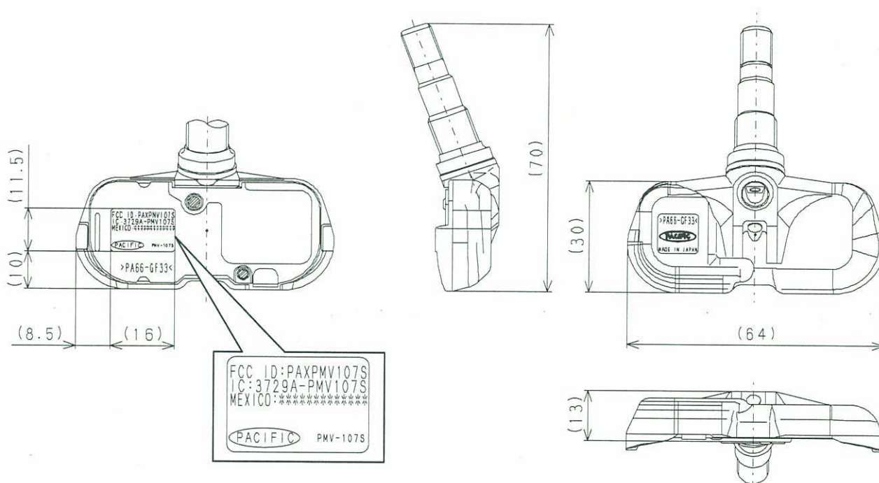
Fig 5. Marking location and dimension
