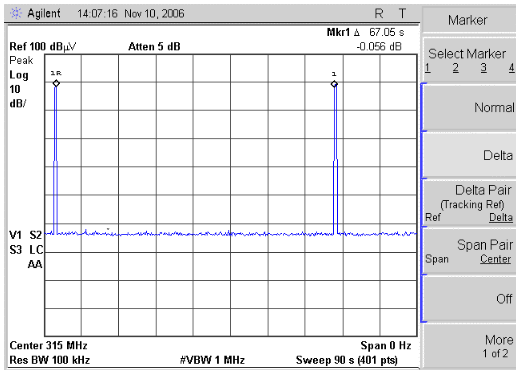
Figure 4. Transmission interval
