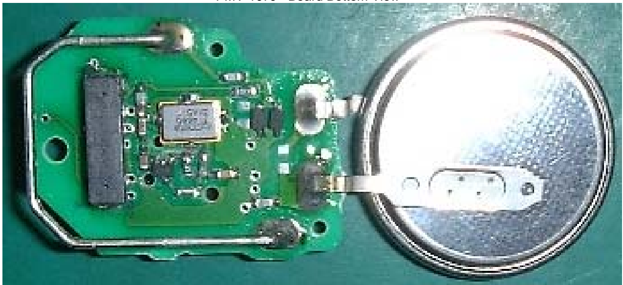
PMV-107J - Board Bottom View
