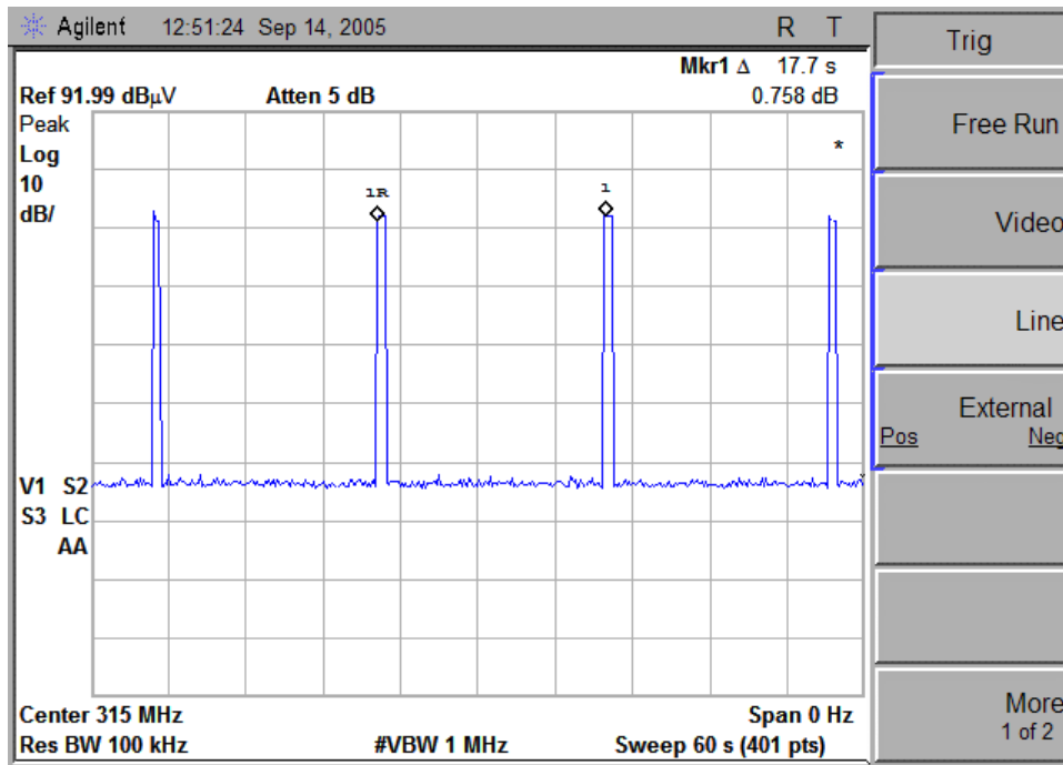
Figure 4. Transmission interval
