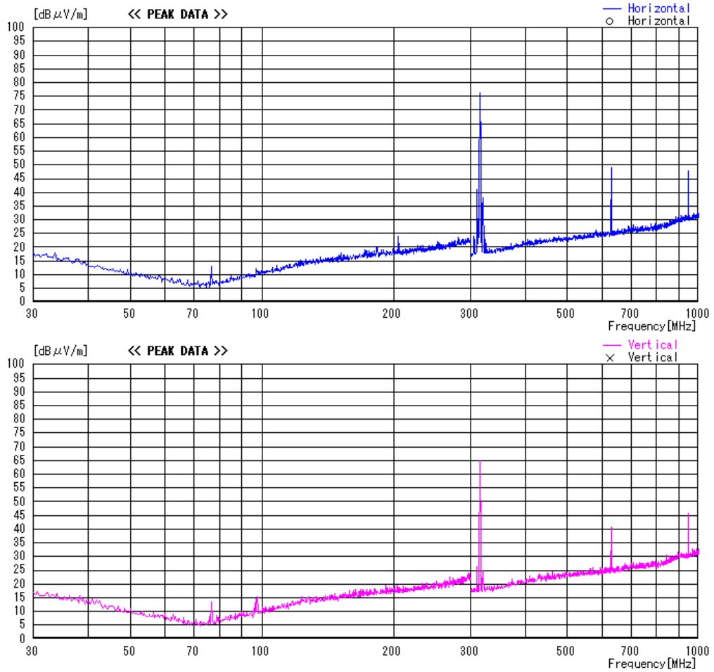
Figure 5. 30-1000MHz spectrum chart
