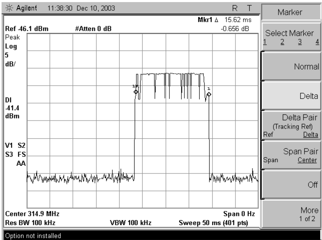
Figure 1. normal transmission
