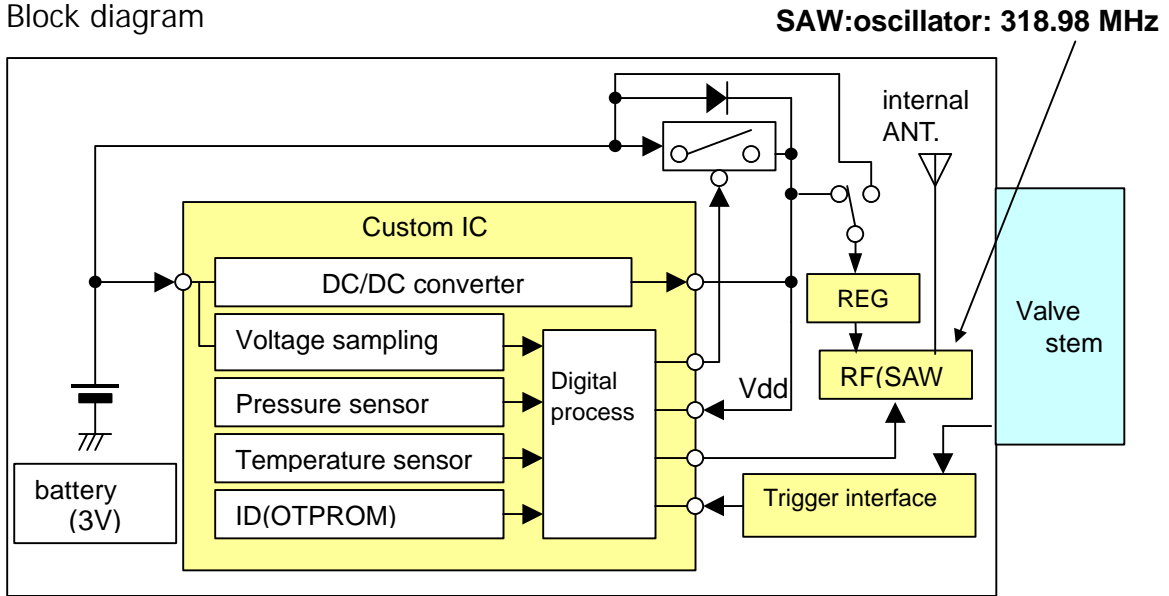
Fig 6, Block diagram of transmitter
