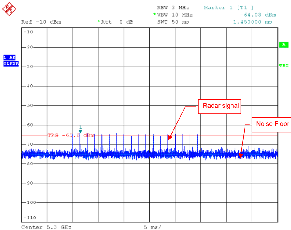
Radar Signal 0
