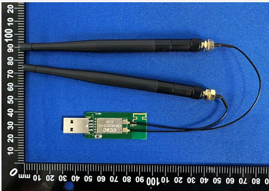
INVAX Antenna
