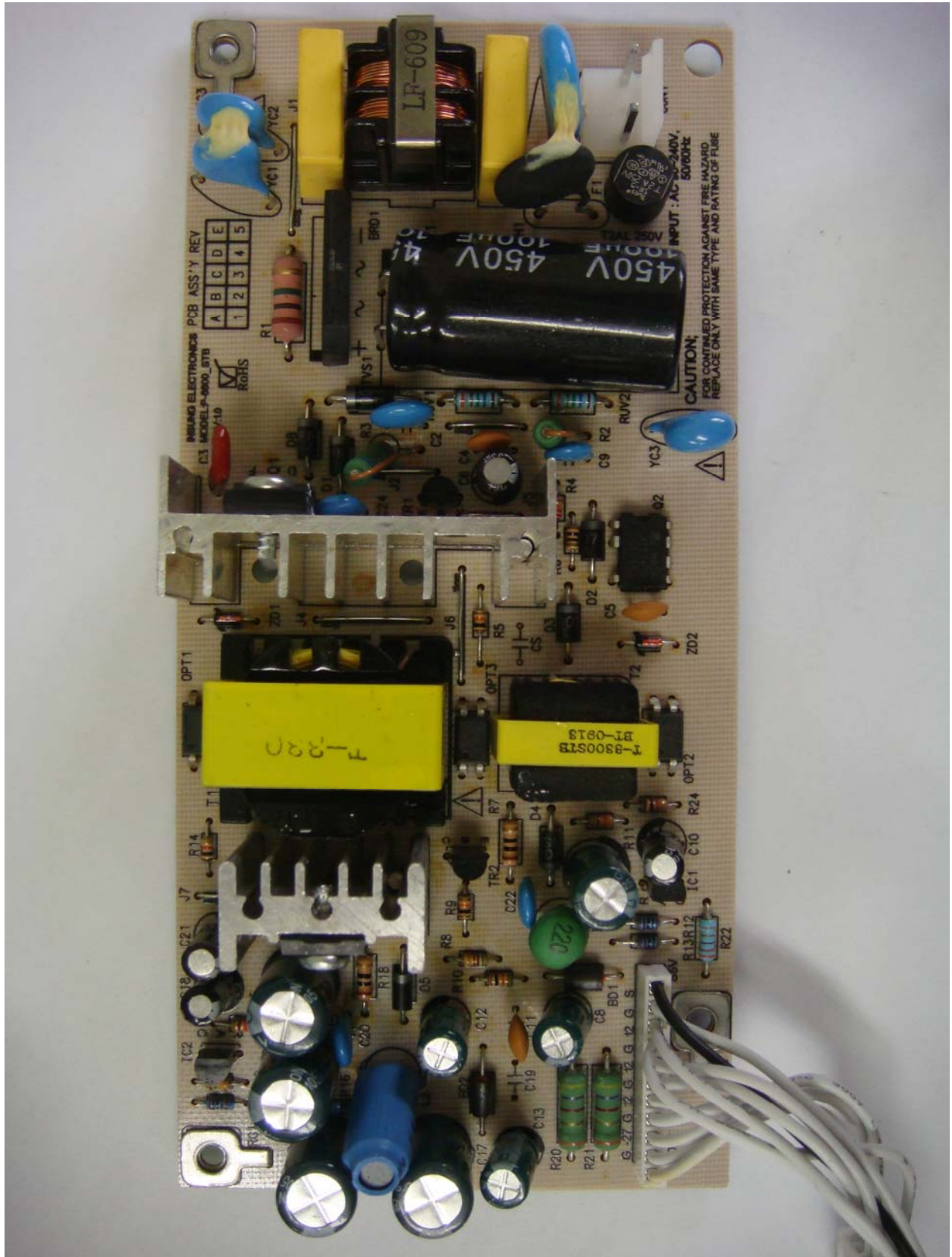
< Photograph 9: AC/DC POWER Board TOP >
