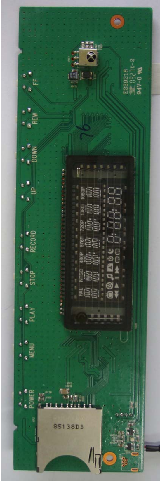
< Photograph 6: LCD Board > TOP
