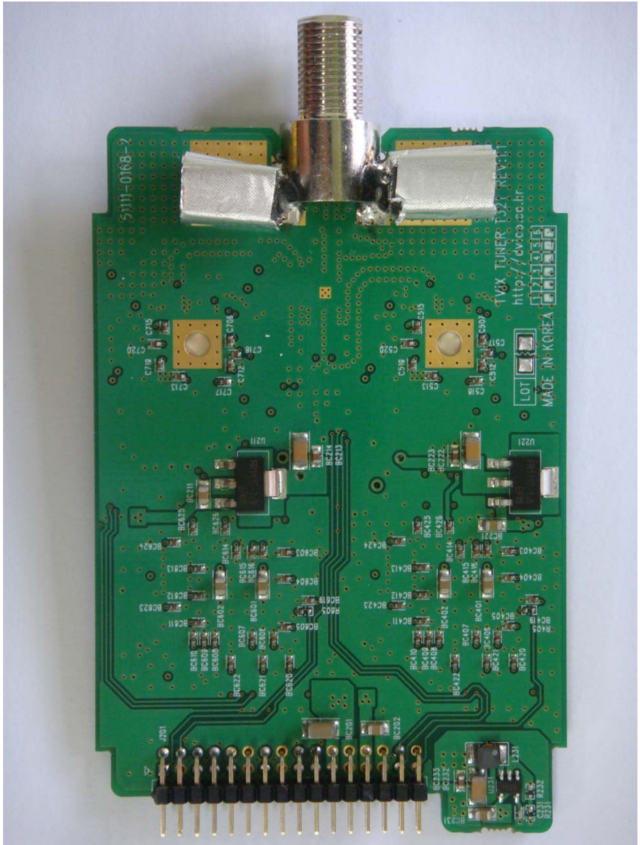
< Photograph 8: Tuner Board BOTTOM >
