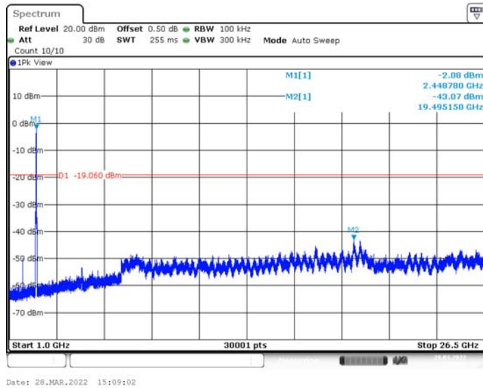
802.11n(HT40)_2452_0~Reference
