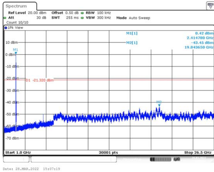
802.11n(HT40)_2437_0~Reference
