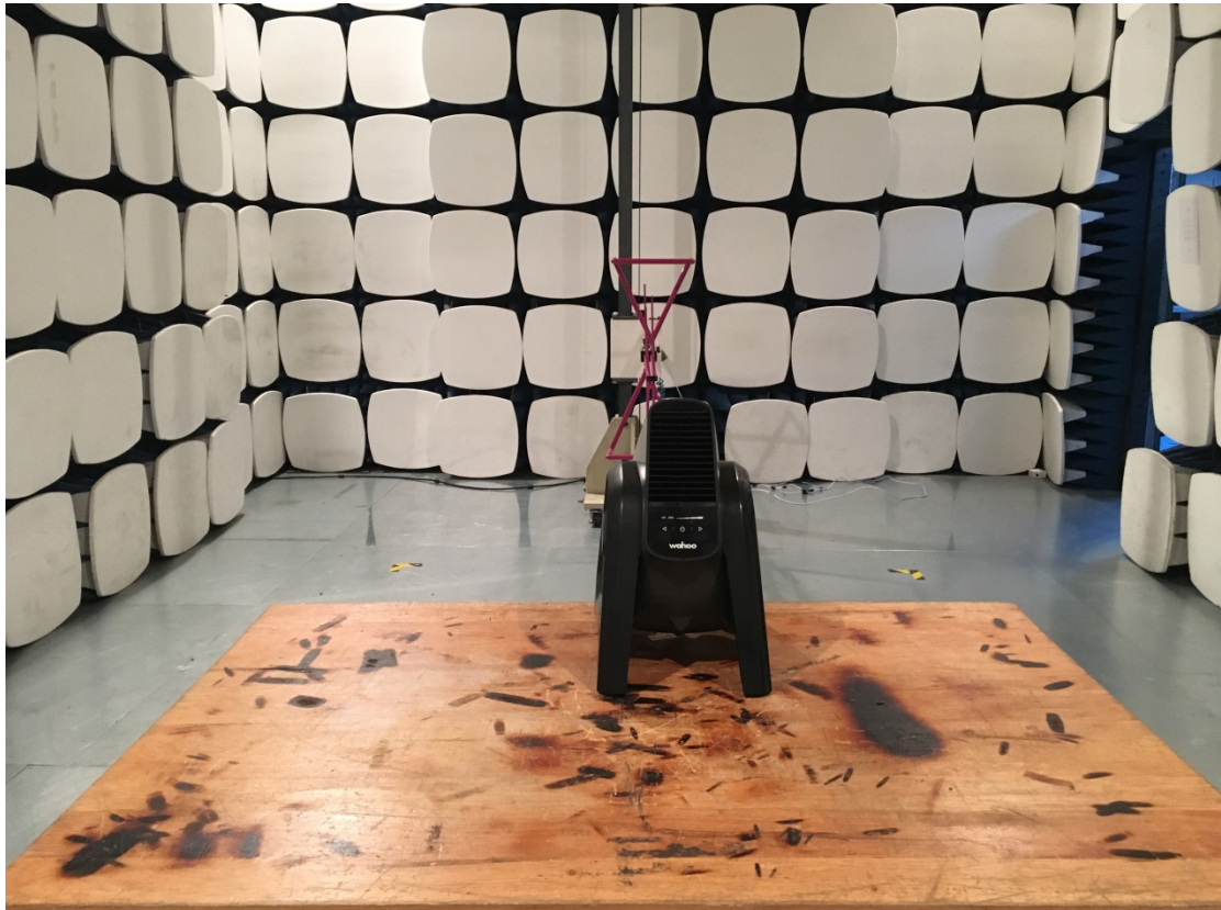
Radiated Emission
