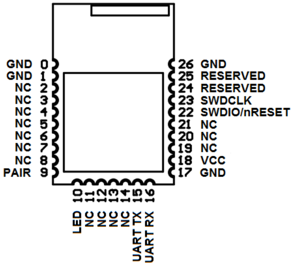
Pinout Diagram
