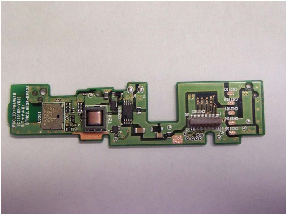
Release PCB Rear
