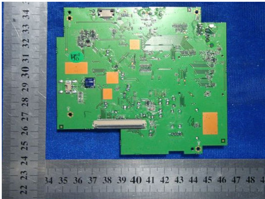
Fig. 6: PCB in photo frame (solder side)
