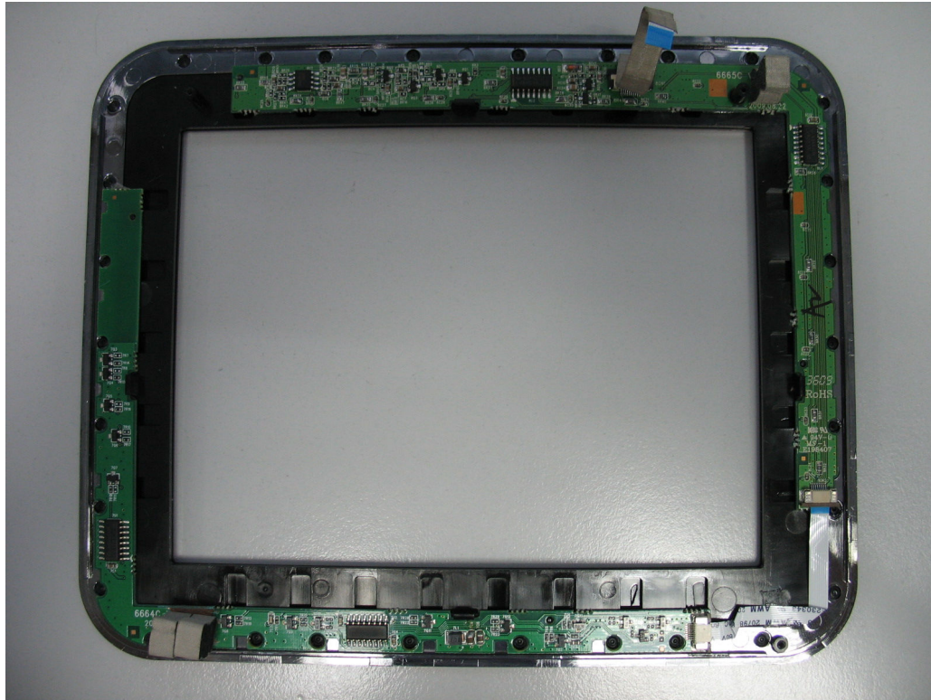
LED PCB
