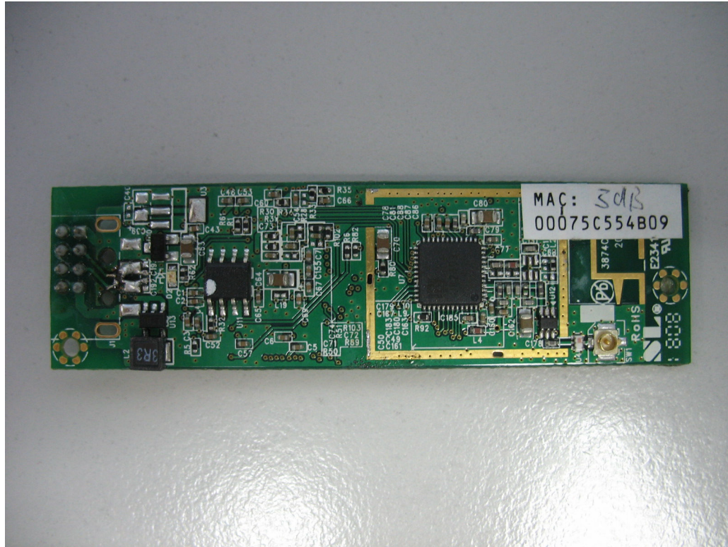
WiFi module PCB (Top)
