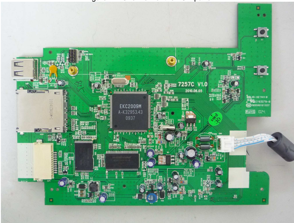
Figure 12. PCB - main board (component side)
