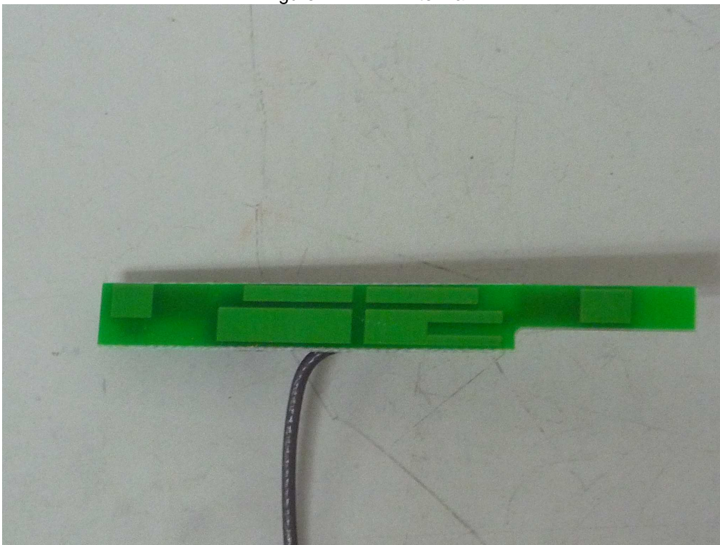
Figure 22. WiFi Antenna
