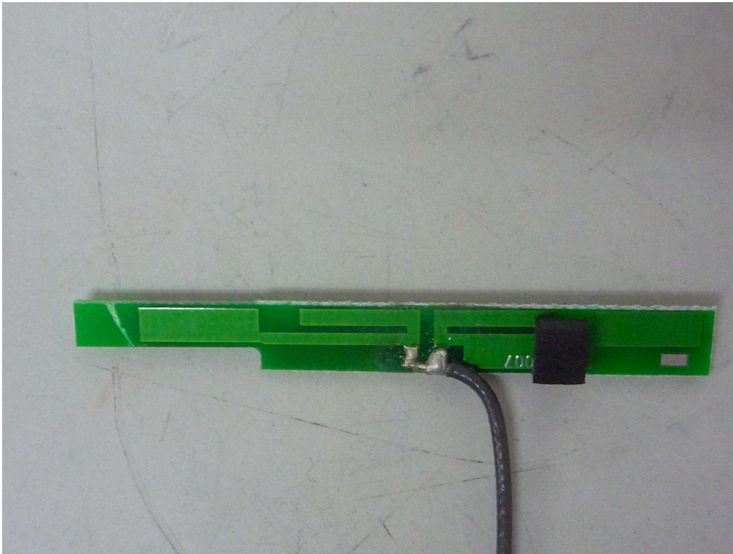
Figure 21. WiFi Antenna
