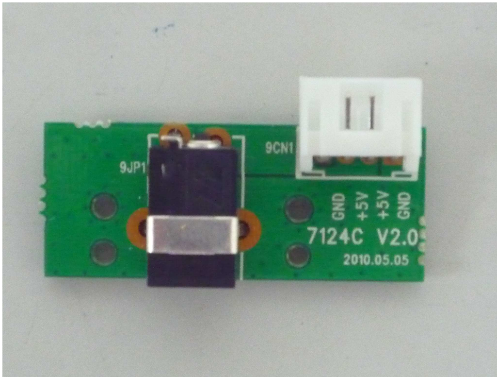
Figure 19. PCB - Power Jack (Top)
