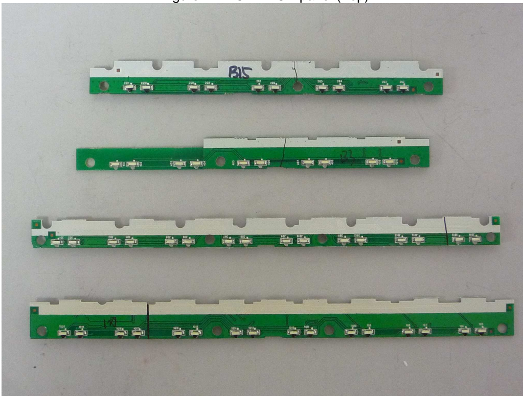
Figure 18. PCB – LCD panel (Bottom)
