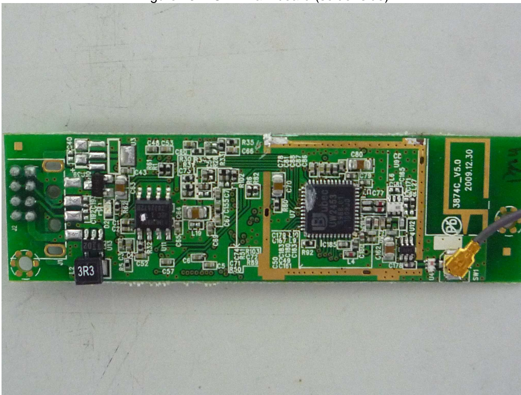
Figure 14. PCB - WiFi module (Top)
