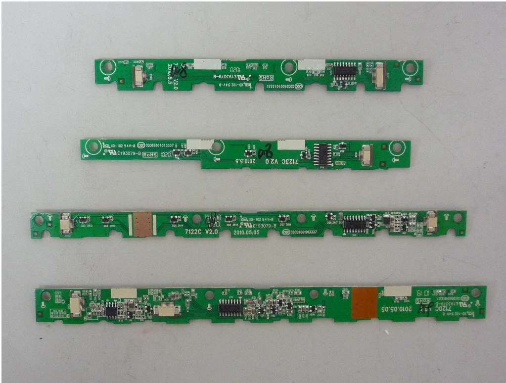
Figure 17. PCB – LCD panel (Top)
