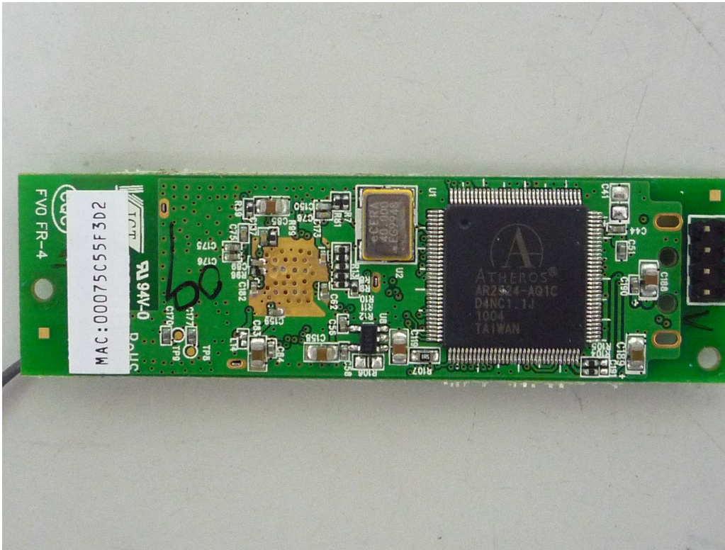
Figure 15. PCB - WiFi module (Bottom)
