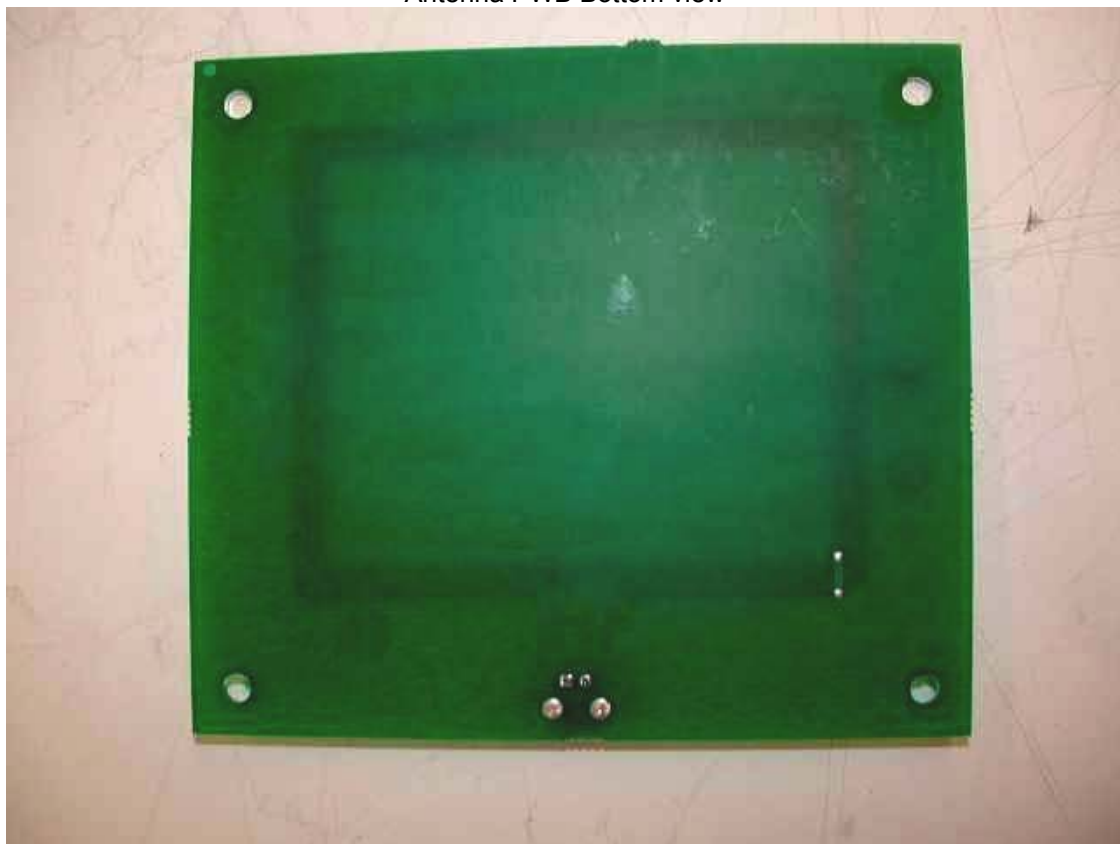
Antenna PWB Bottom view
