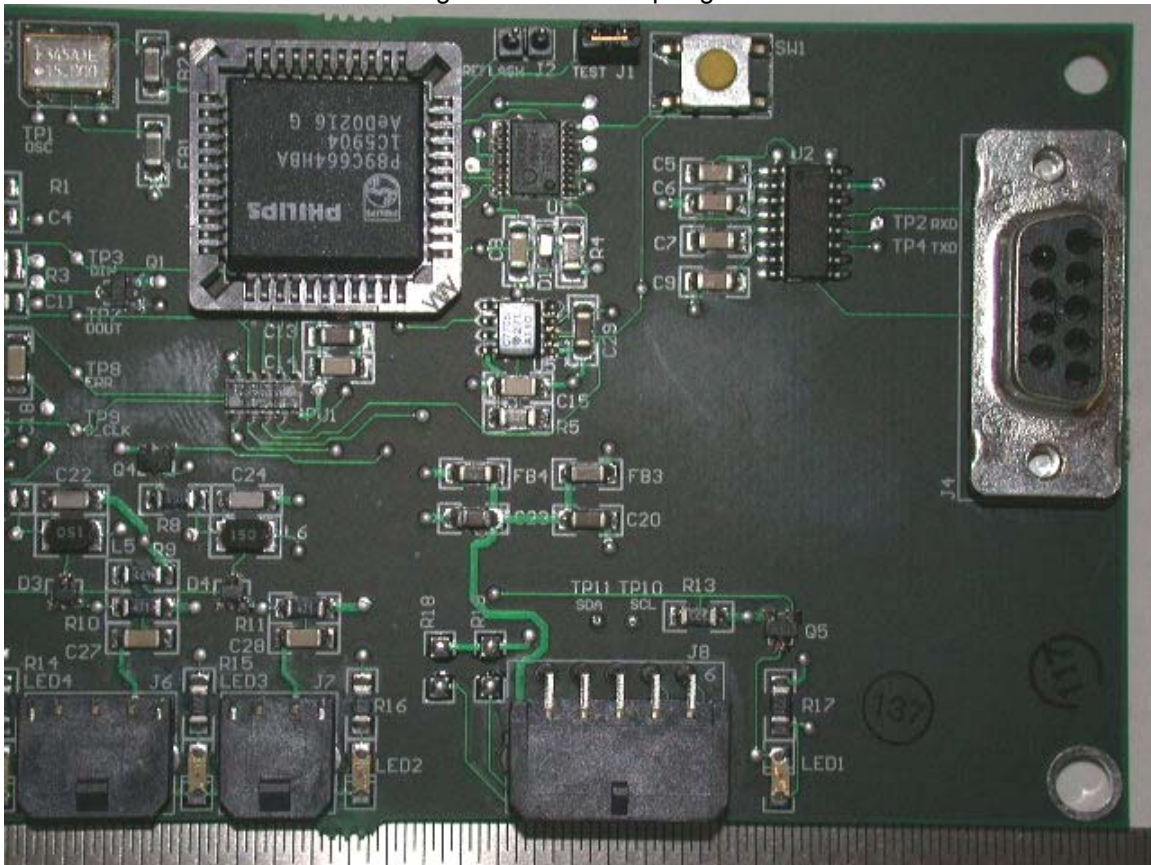
RF Tag Reader PWB Top Right view
