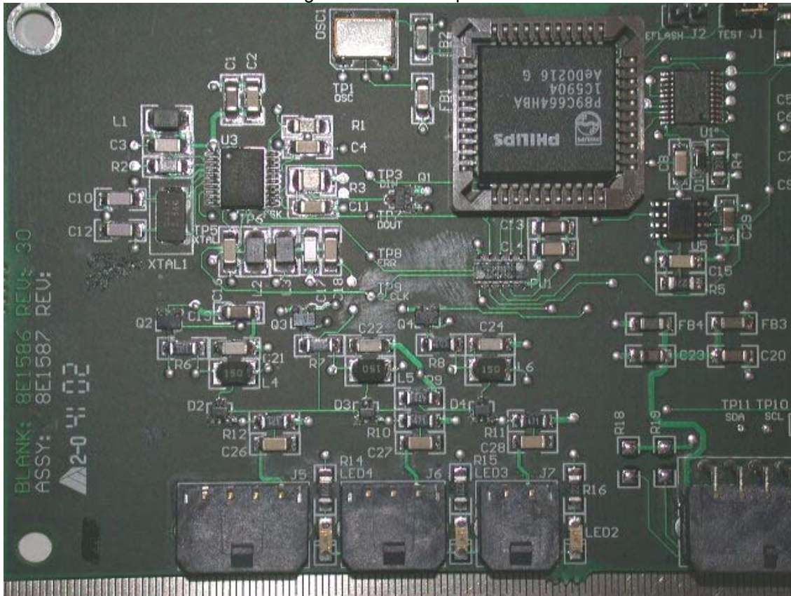
RF Tag Reader PWB Top Left view
