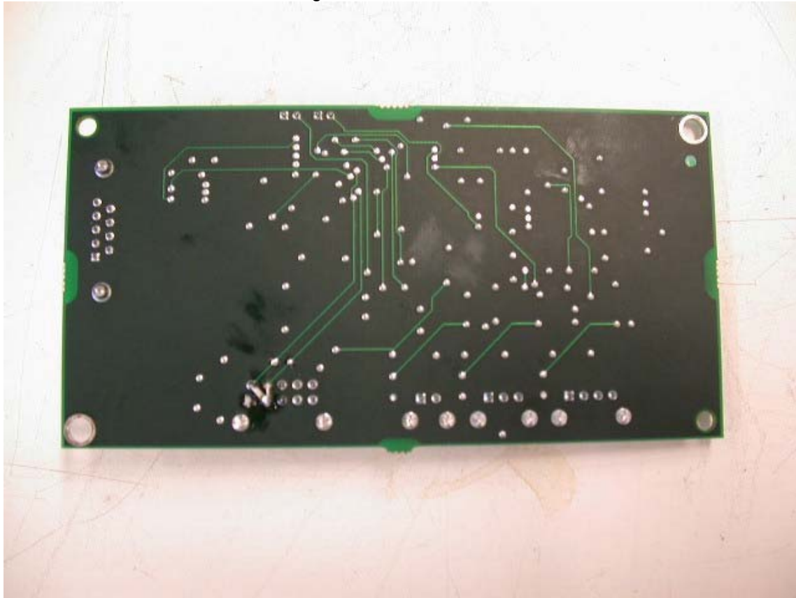
RF Tag Reader PWB Bottom view
