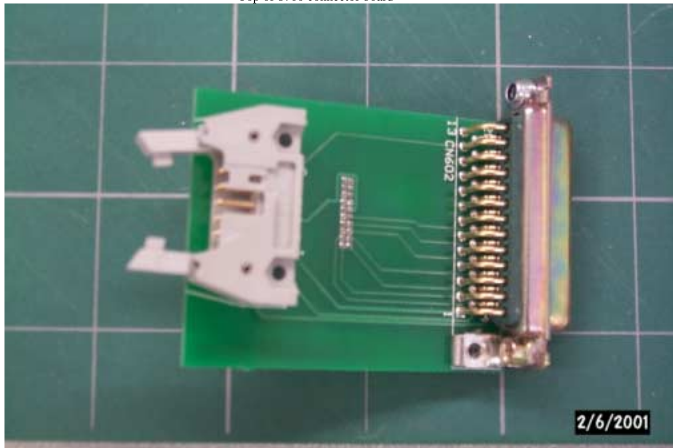
Top of 8700 connector board
