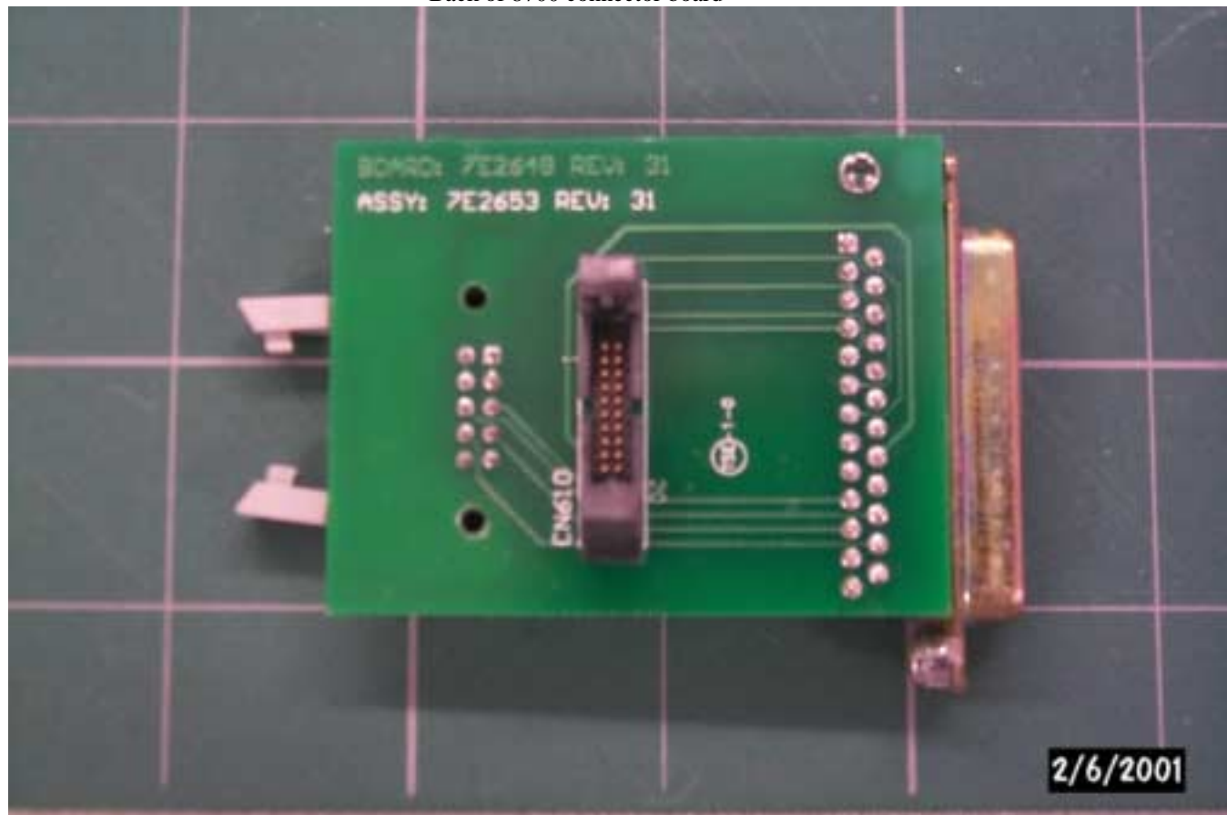
Back of 8700 connector board
