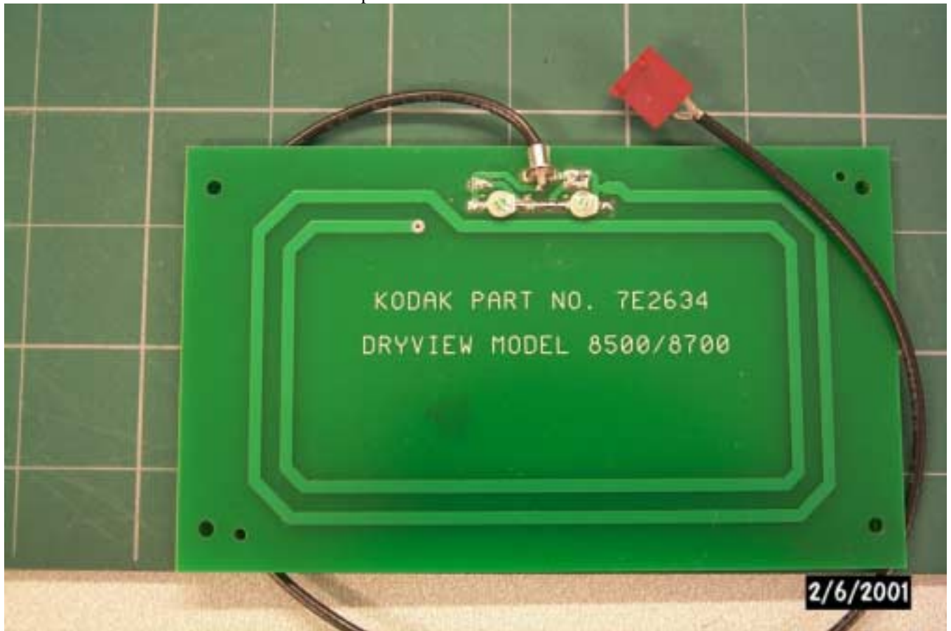
Top of 8700 antenna board
