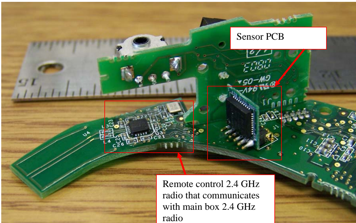
Kodak remote PCB with 2.4 GHz radio and sensor PCB identified
