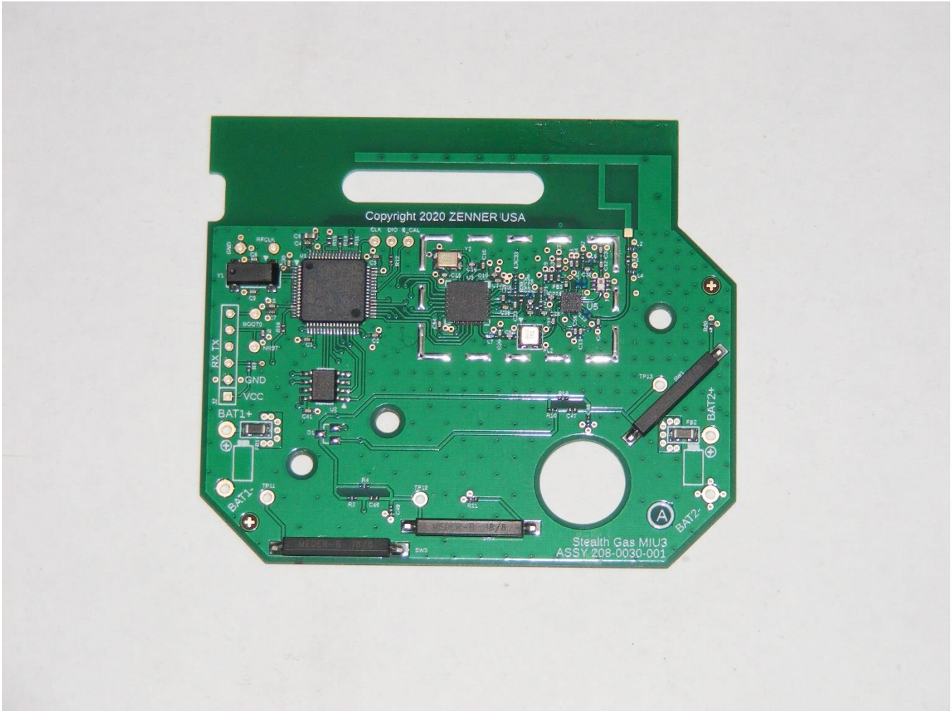
Figure 2: RFG-301 PCB – Top
