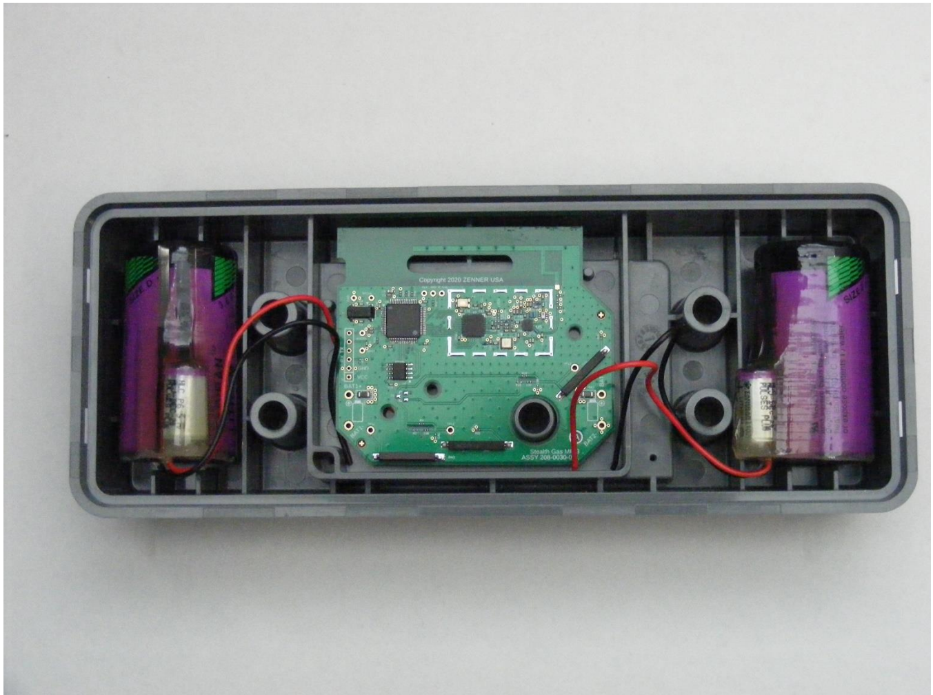
Figure 1: RFG-301 Internal View
