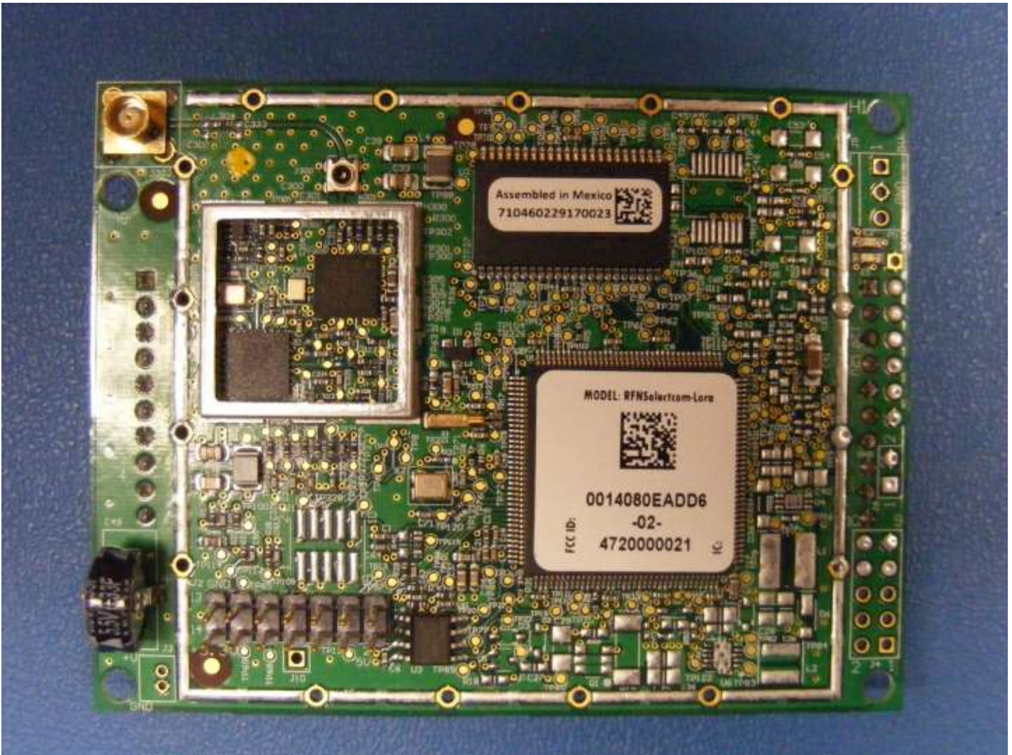
Figure 3: RFN SelectComm 1272 (3.3V) – Top, shield removed
