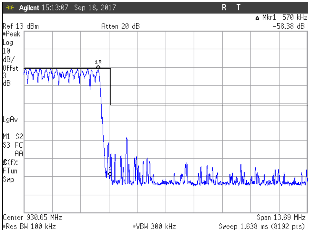
Figure 44: Band-edge, Hopping Mode, Upper Band Edge, Low Power Setting
