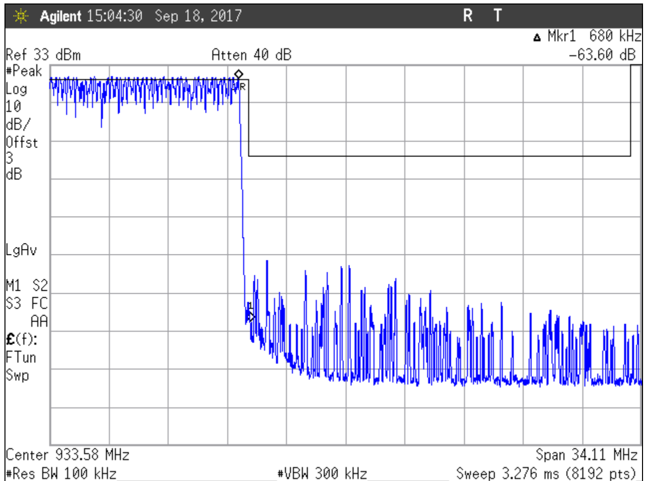
Figure 40: Band-edge, Hopping Mode, Upper Edge, High Power Setting
