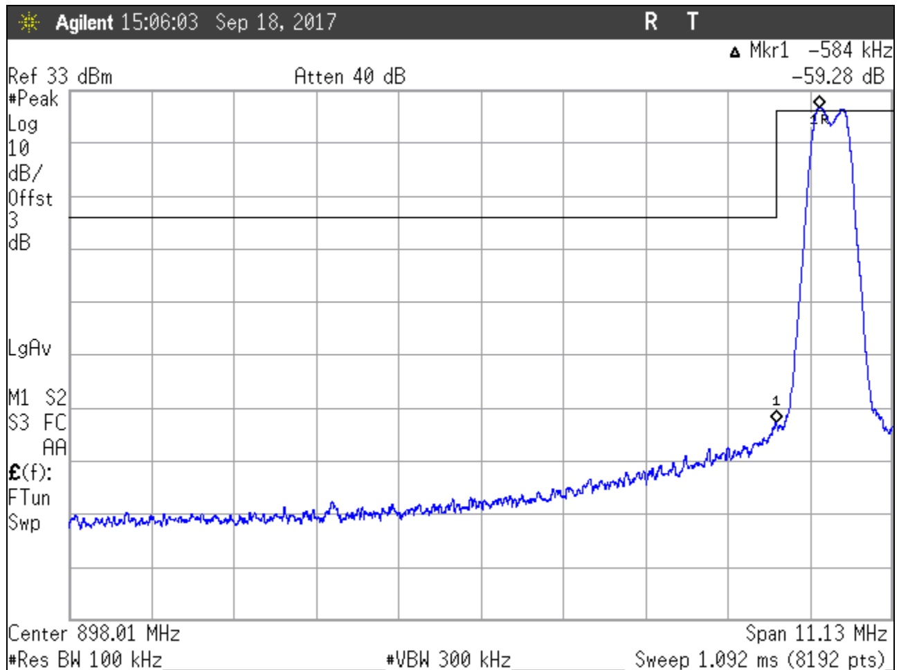
Figure 41: Low Channel, Lower Band-edge, High Power Setting
